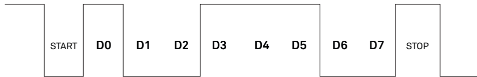
Figure 10 Example DDI serial transmission of the character 9 (0x39)
